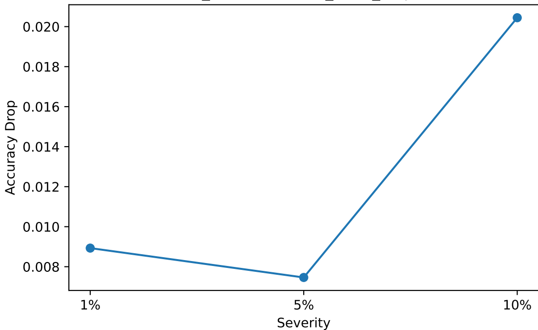
hhar Flatten_LSTM classifier_head_only calibration
