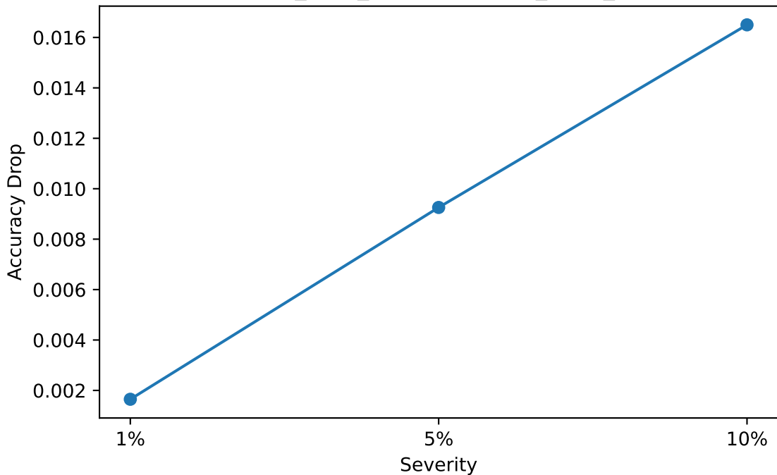
pamap2 Improved_GNN_LSTM classifier_head_only calibration
