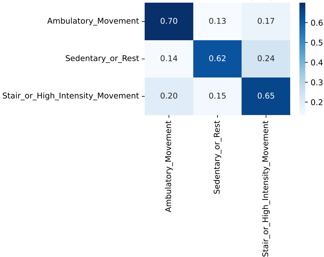
hhar CNN1D health groups
