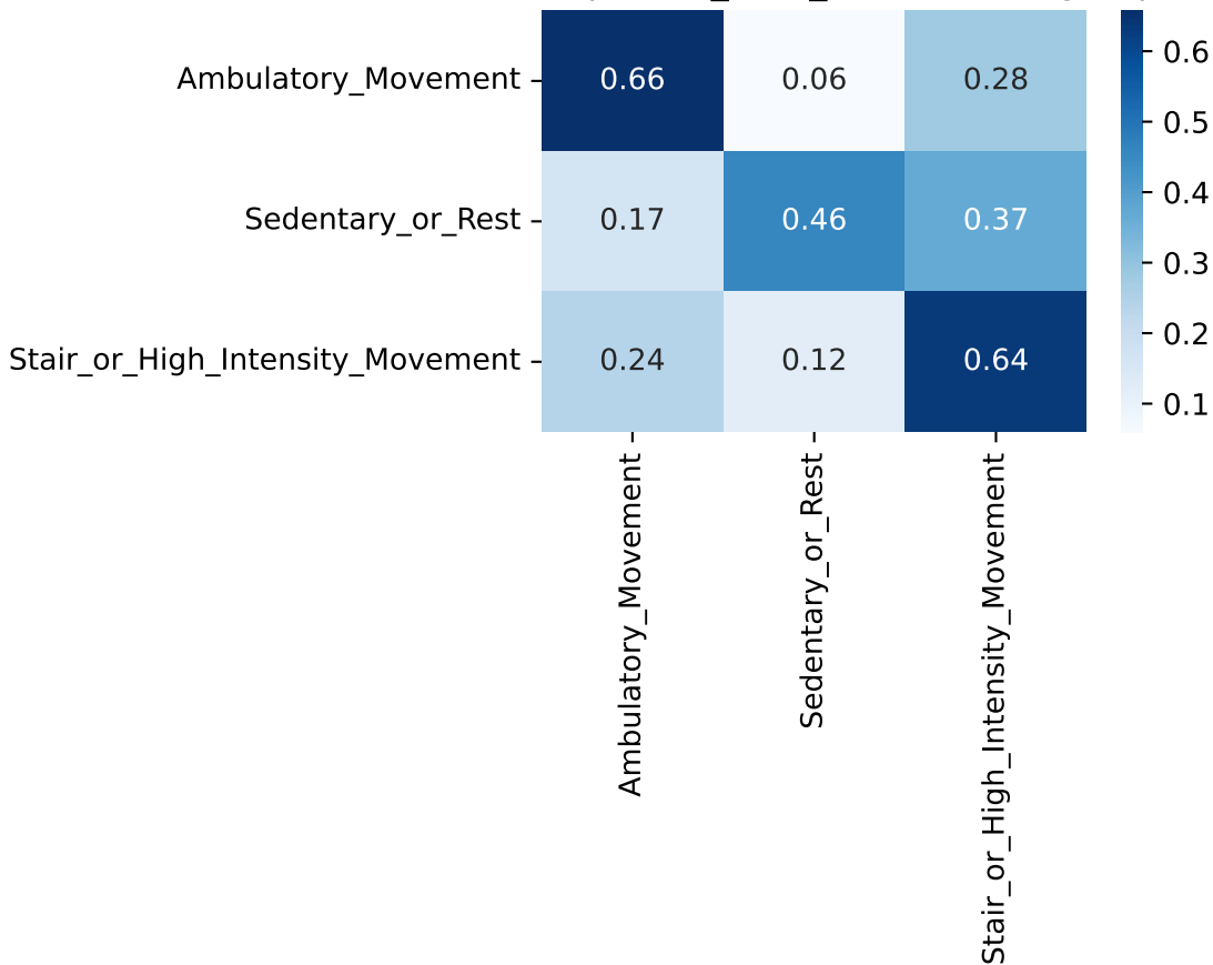
hhar Improved_GNN_LSTM health groups
