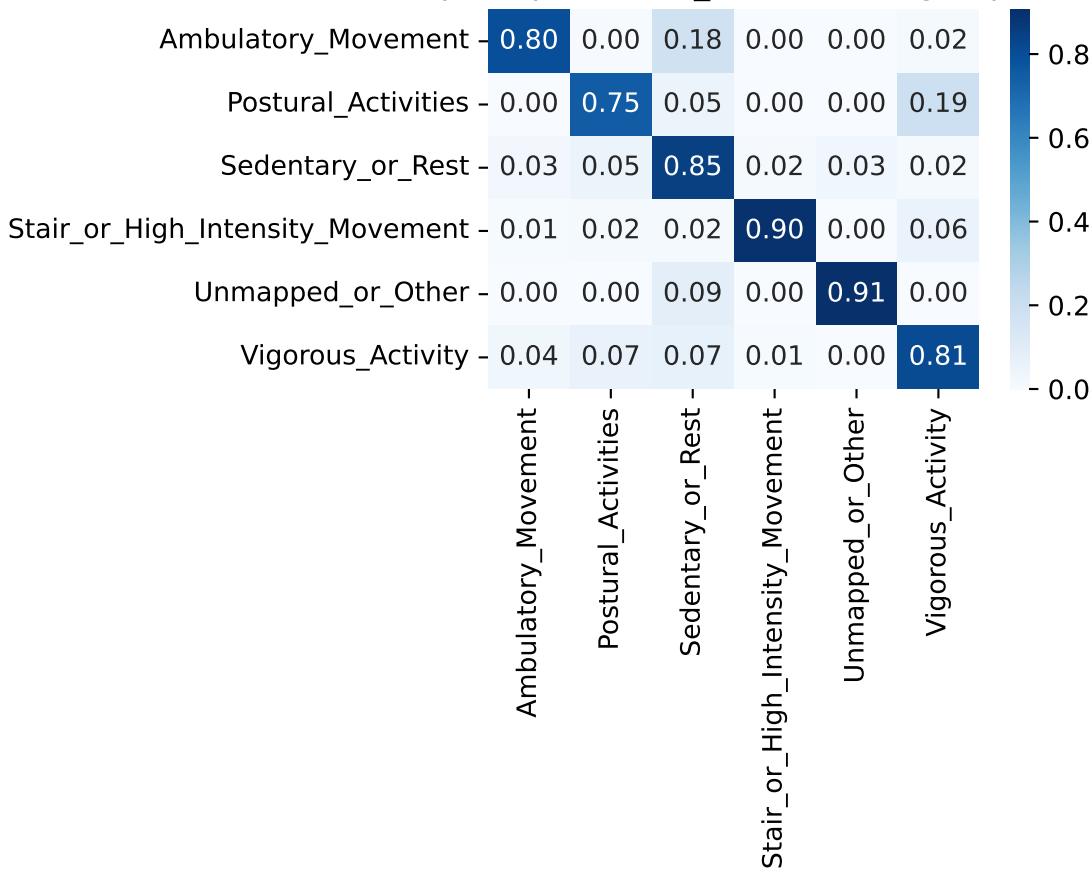
pamap2 Flatten_LSTM health groups
