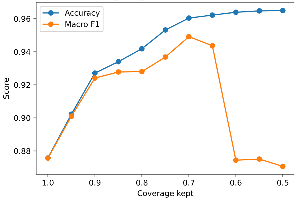
Selective Prediction: acc16_gyro_hr / overlapping / Improved GNN-LSTM Res
