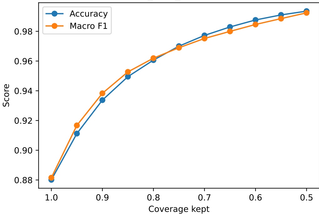
Selective Prediction: acc16_gyro_hr / overlapping / Random Forest
