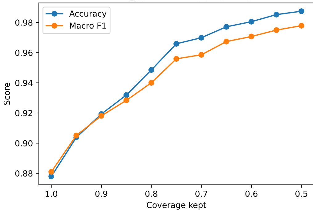
Selective Prediction: acc16_gyro / overlapping / Improved AttnAdj ResBN
