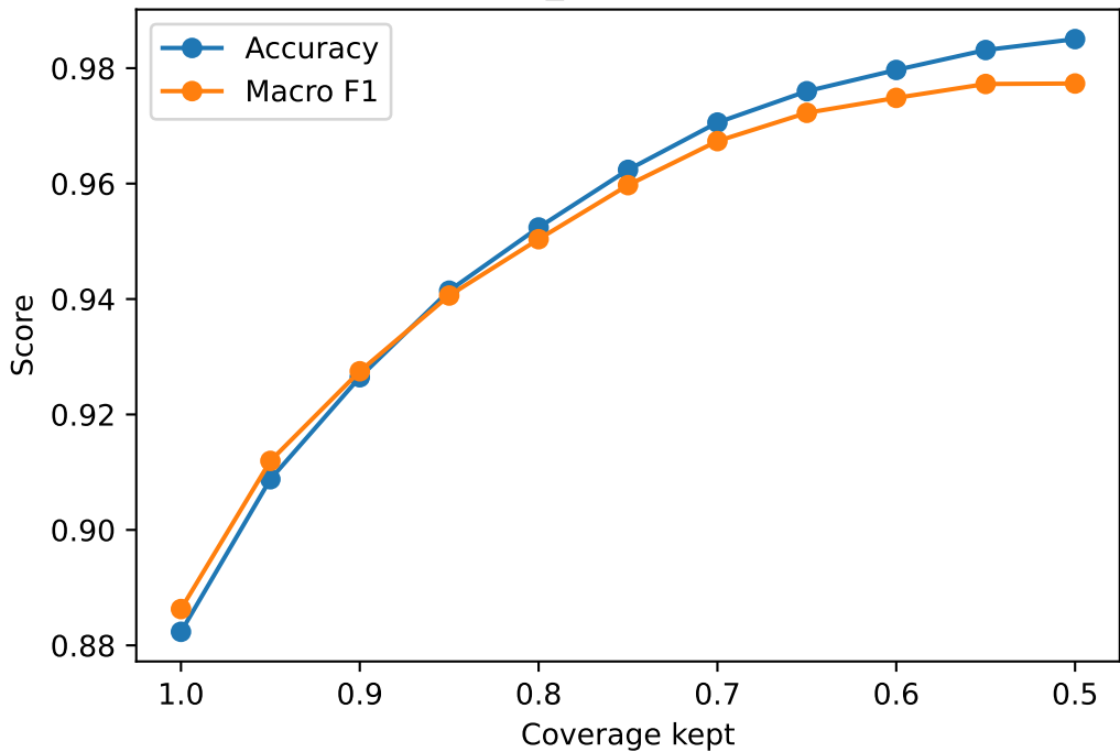
Selective Prediction: acc16_gyro / overlapping / Random Forest
