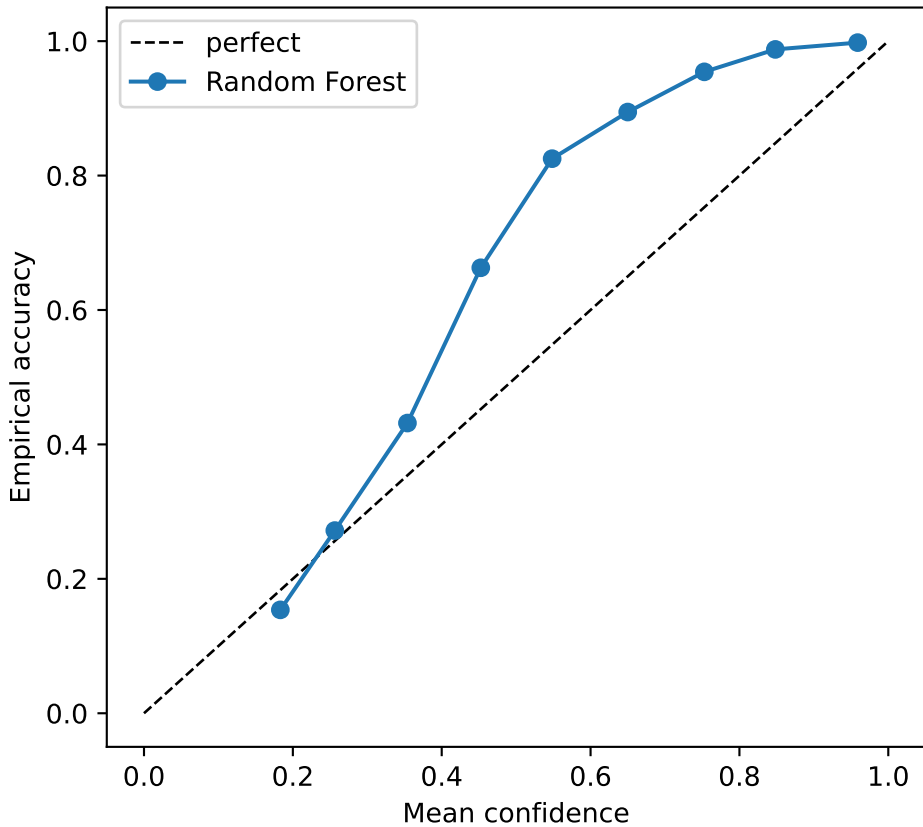
Reliability: acc16_gyro_hr / overlapping / Random Forest
