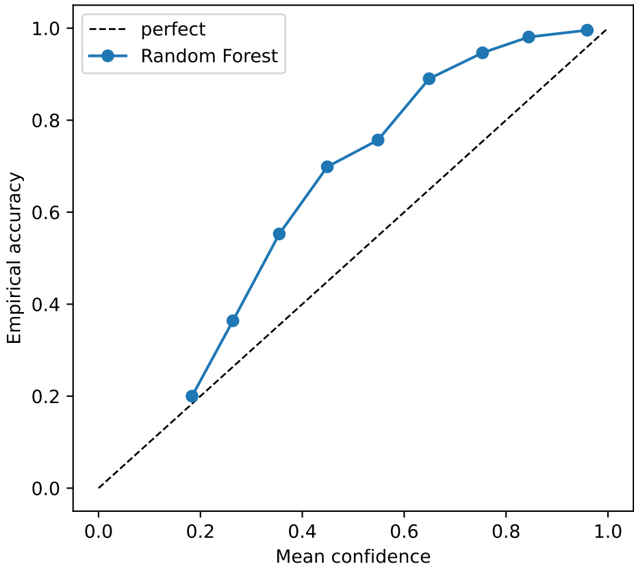
Reliability: acc16_gyro / non_overlapping / Random Forest
