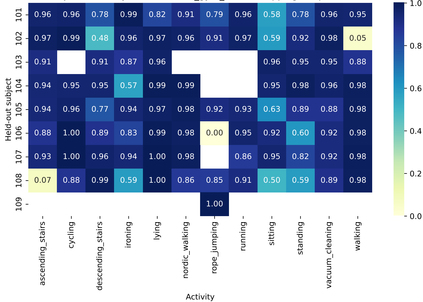
Experiment 5: Subject x Activity Recall - acc16_gyro_hr / overlapping / Improved GNN-LSTM Res
