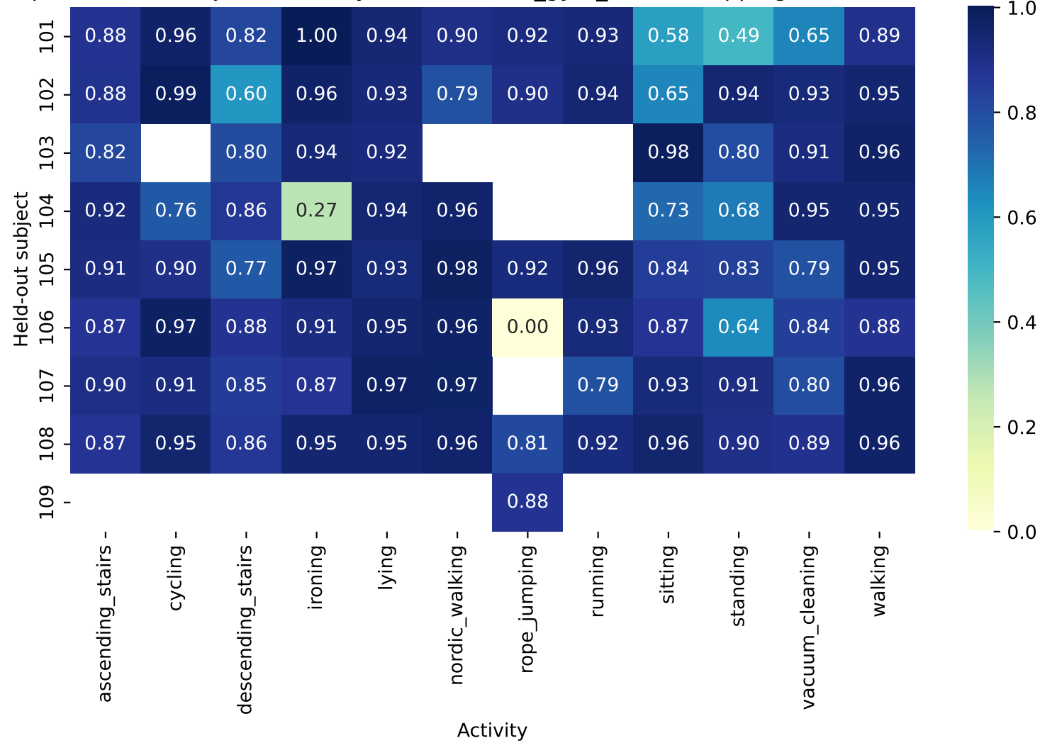
Experiment 5: Subject x Activity Recall - acc16_gyro_hr / overlapping / Random Forest
