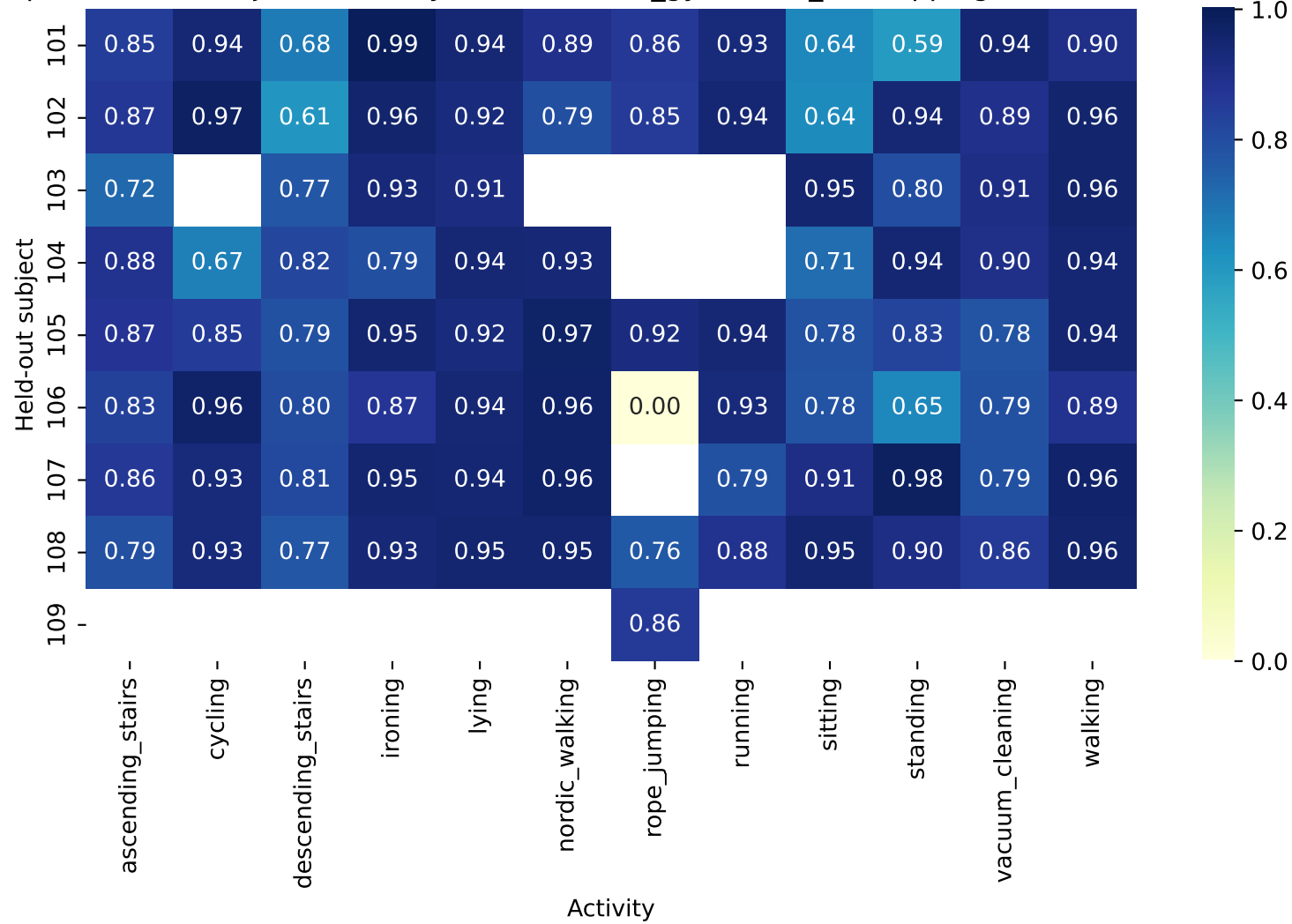
Experiment 5: Subject x Activity Recall - acc16_gyro / non_overlapping / Random Forest
