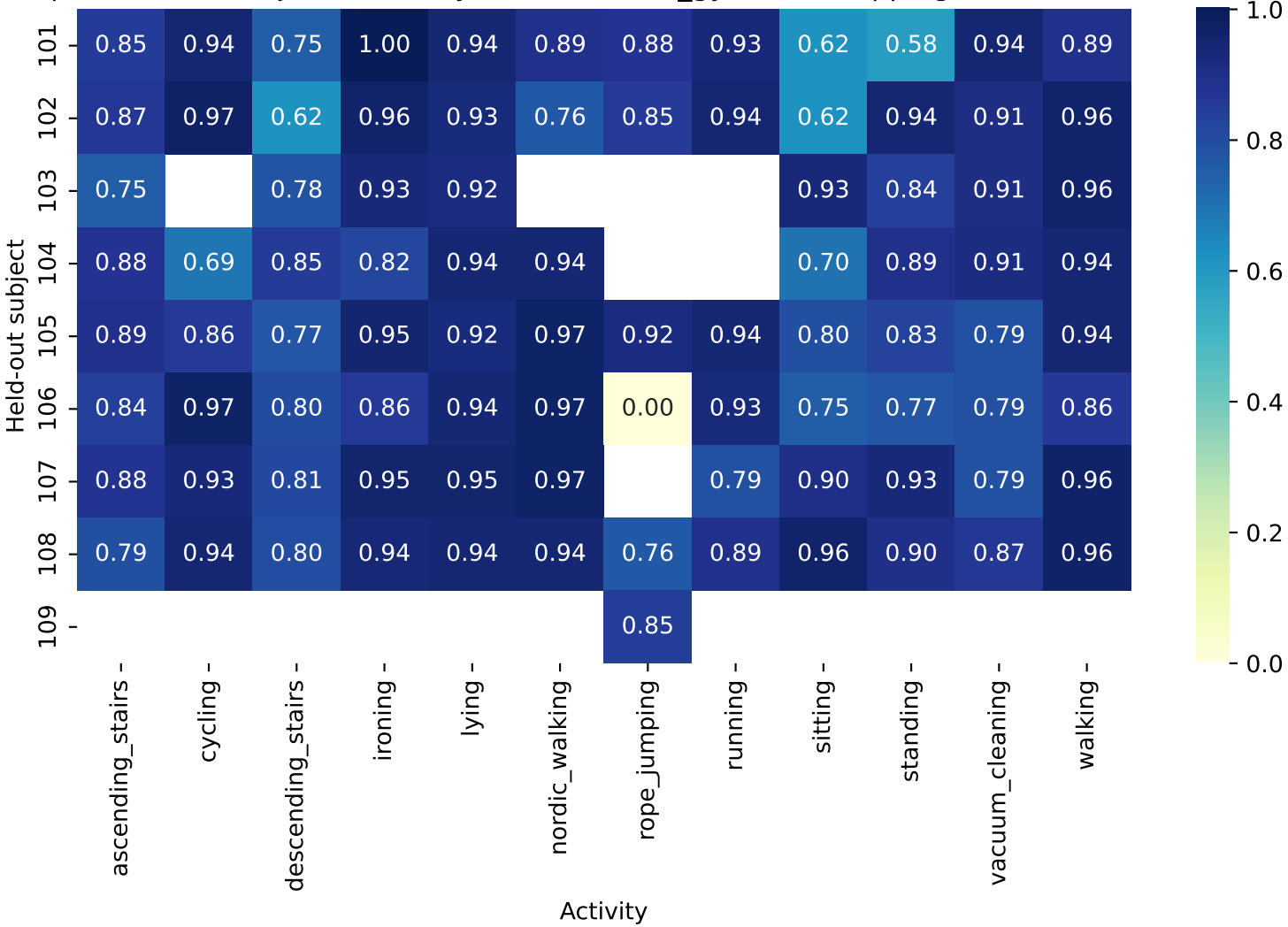
Experiment 5: Subject x Activity Recall - acc16_gyro / overlapping / Random Forest
