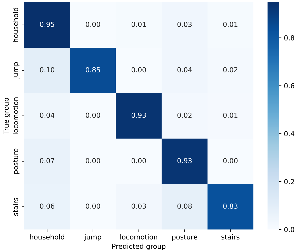
Experiment 7: Health Group Confusion - acc16_gyro / non_overlapping / Random Forest
