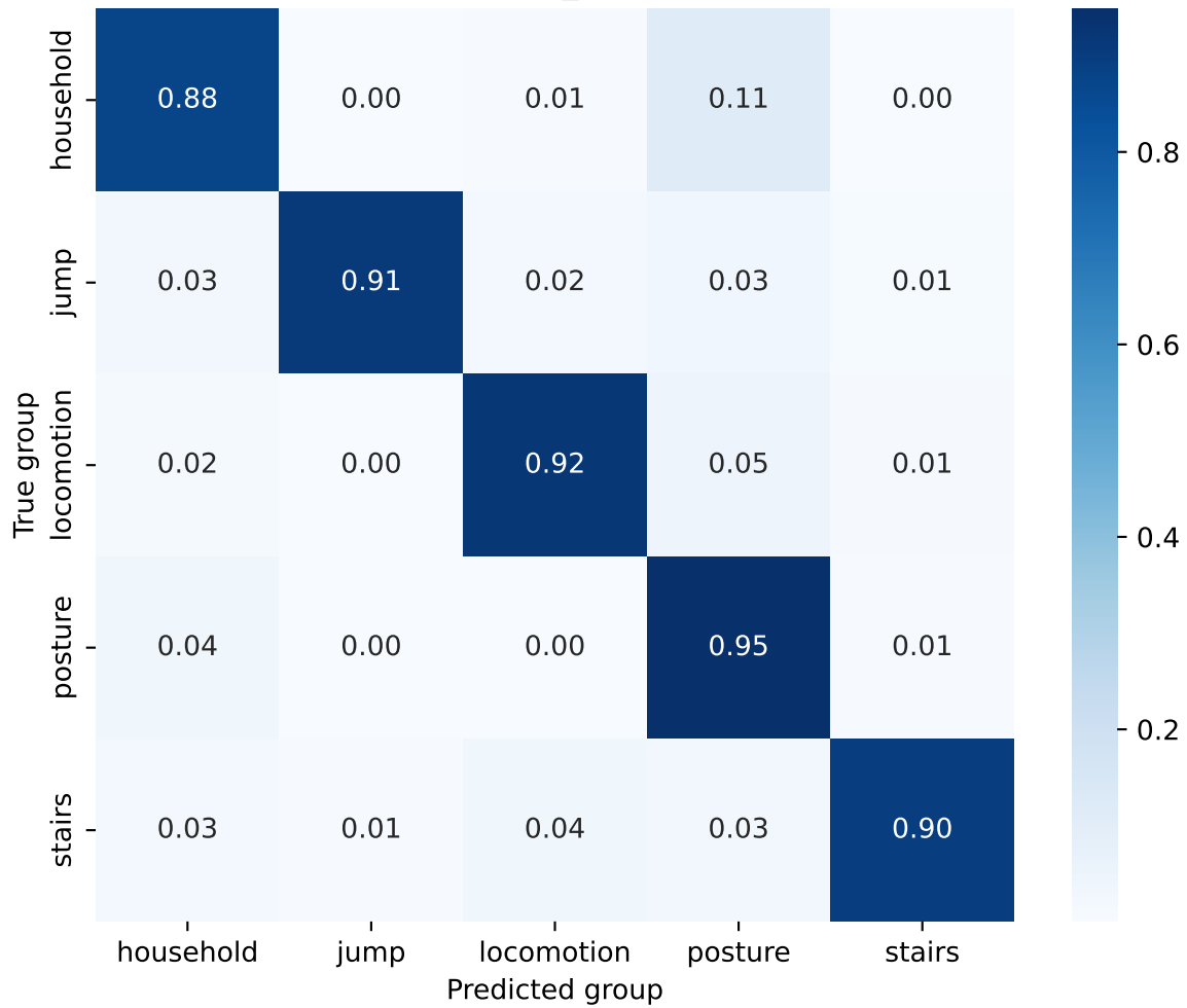
Experiment 7: Health Group Confusion - acc16_gyro / overlapping / Improved AttnAdj ResBN
