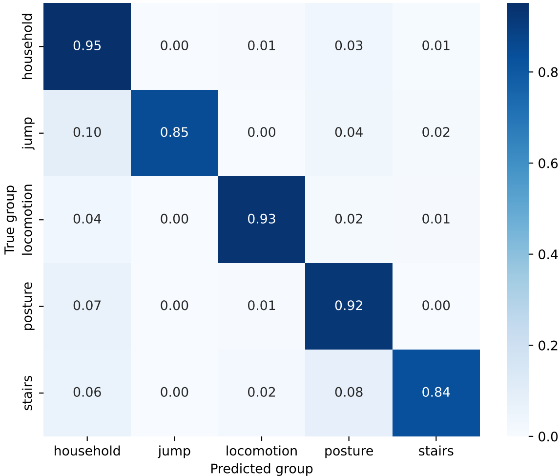
Experiment 7: Health Group Confusion - acc16_gyro / overlapping / Random Forest
