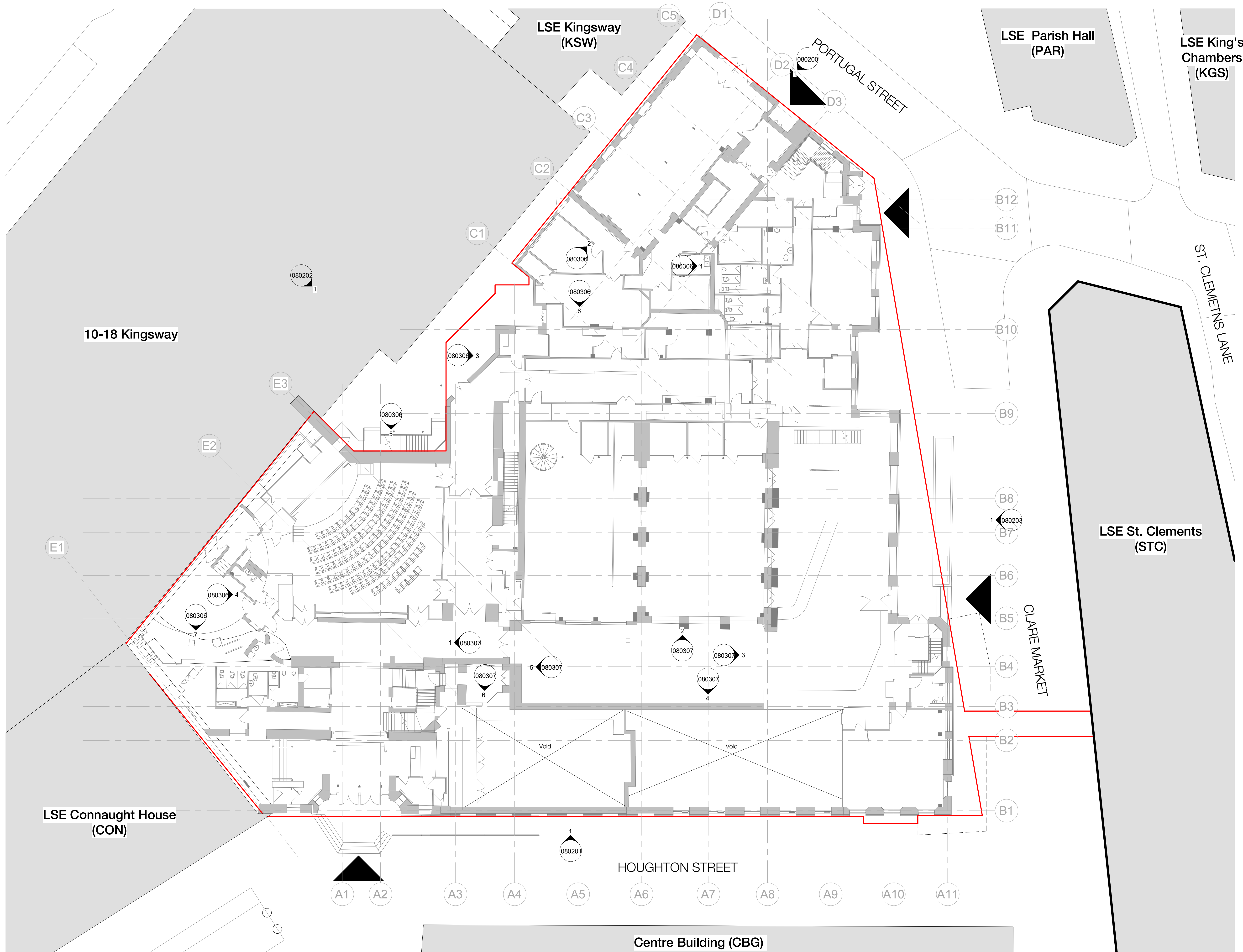
Ground Floor Plan - Existing & Strip-out 1 : 150
