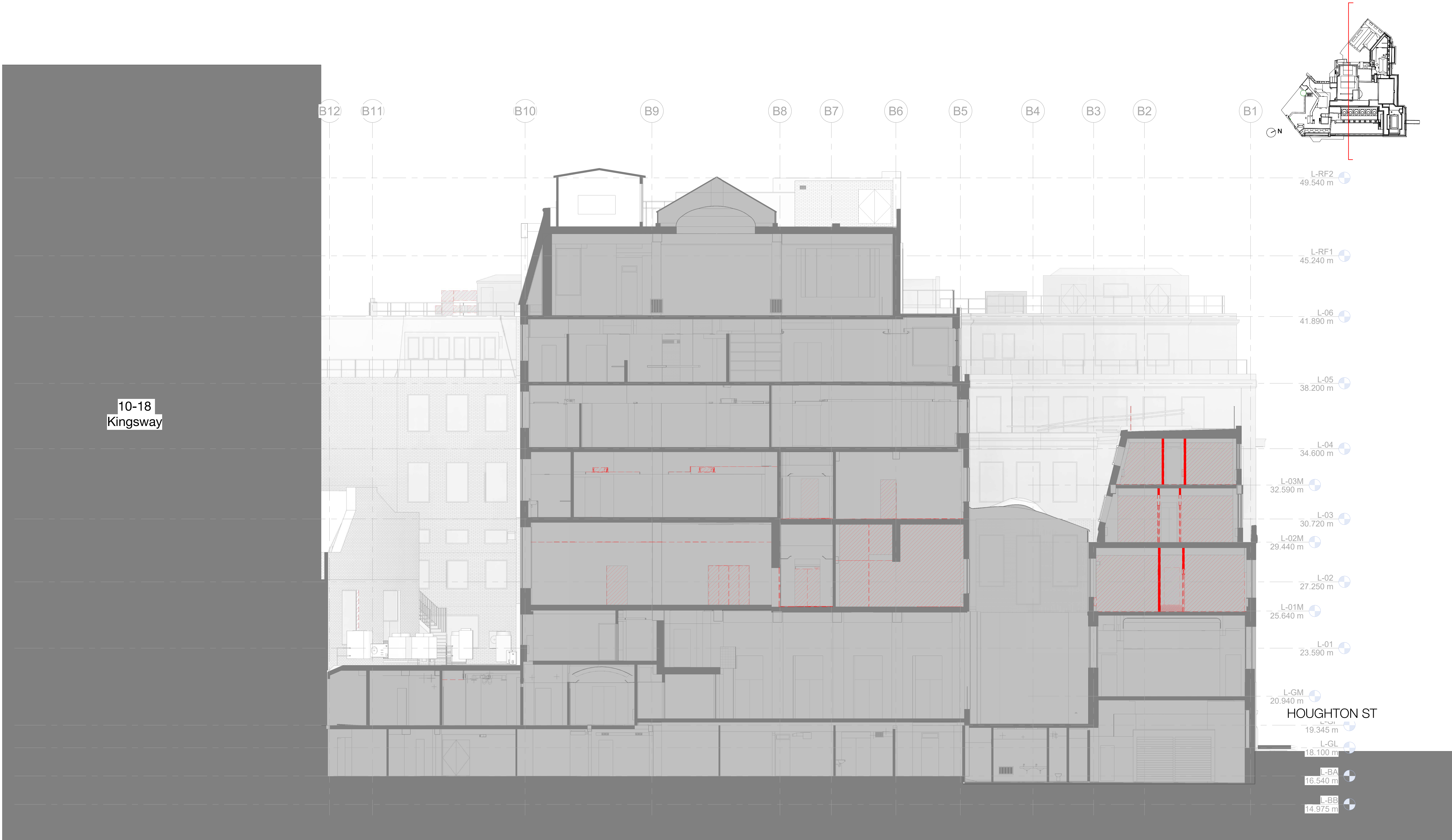
Section AA - Existing & Strip-out 1 : 100
