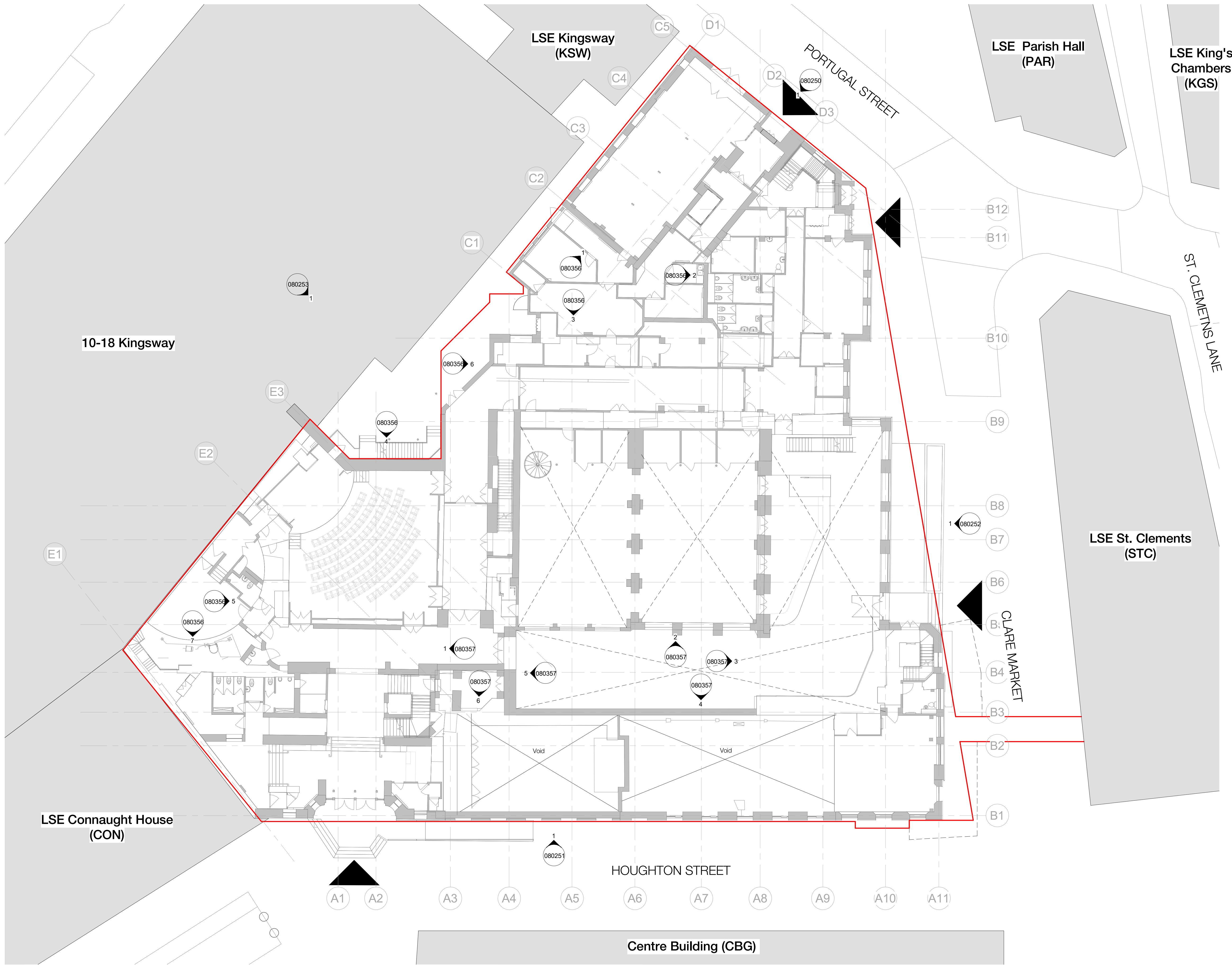
Ground Floor Plan - Proposed 1 : 150
