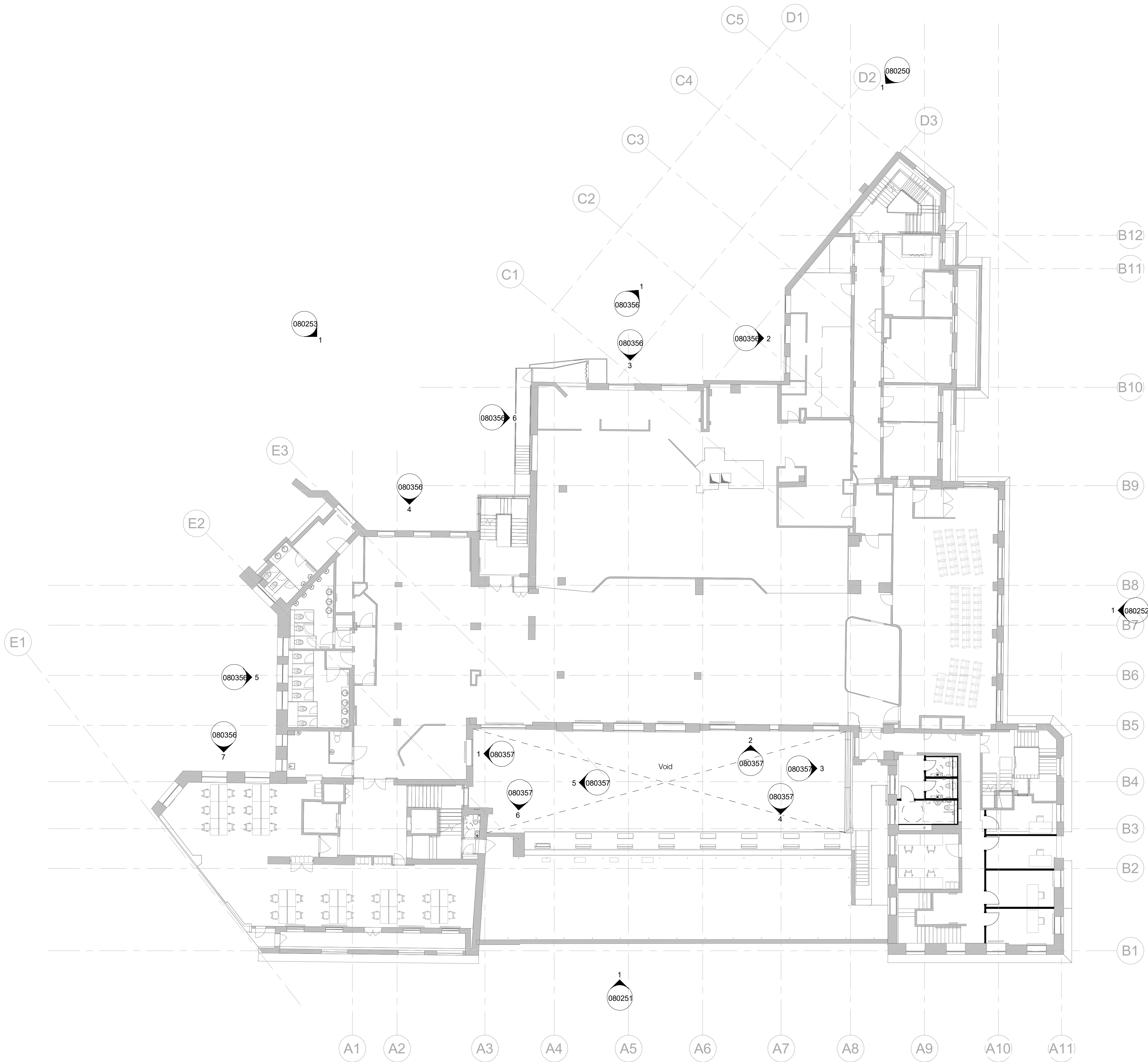
Fourth Floor Plan - Proposed 1 : 150
