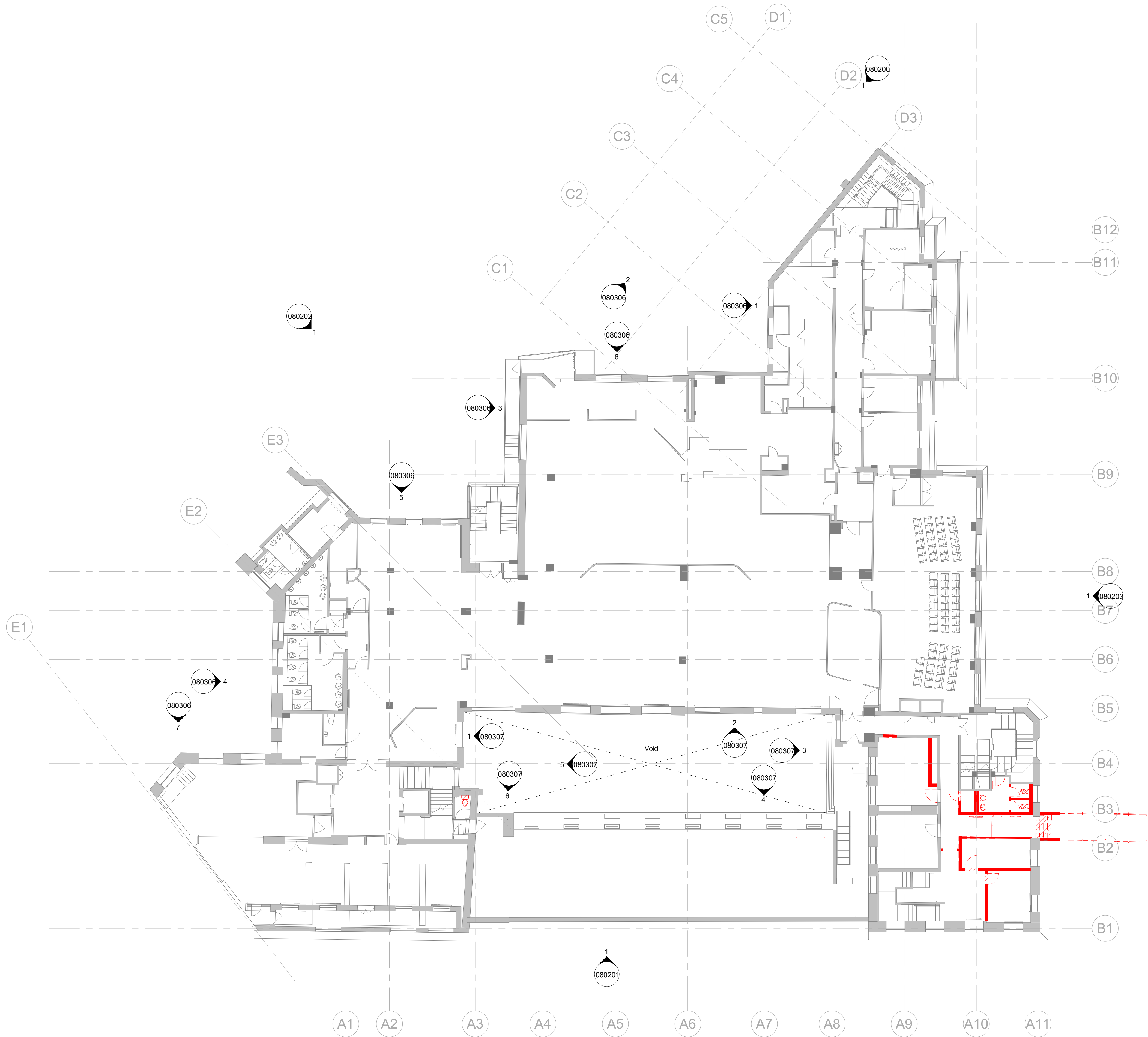
Fourth Floor Plan - Existing & Strip-out 1 : 150
