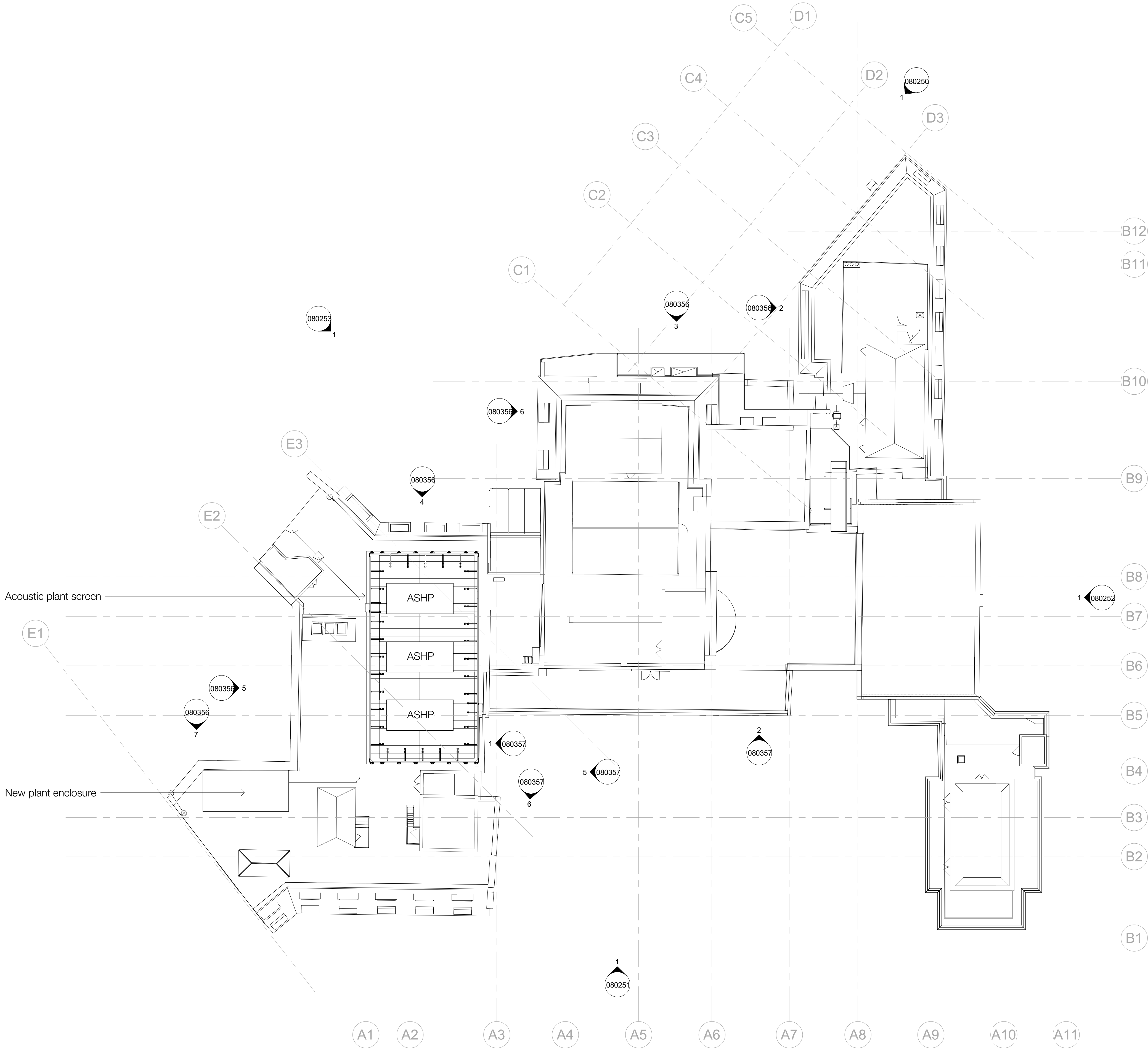
Roof Plan - Proposed 1 : 150
