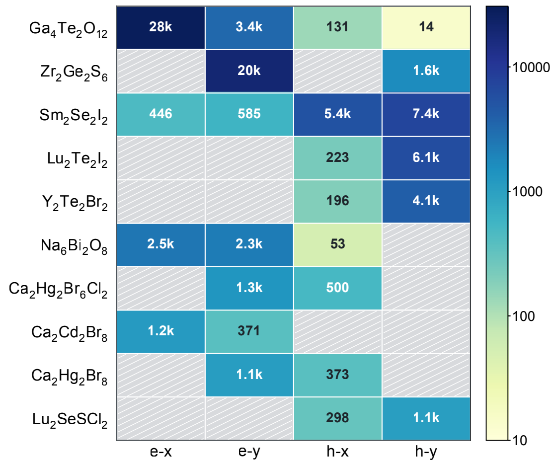
b Reliability-gated DFT mobility heatmap (25 channels / 10 materials)
