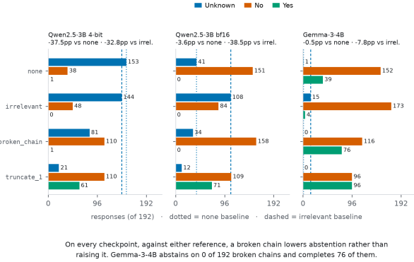
Figure 4: Three-candidate response distribution, three checkpoints, four arms. Dotted and dashed lines mark the NONE and IRRELEVANT abstention baselines, 4.7pp apart at 4-bit and 34.9pp at bfloat16. A broken chain lowers abstention against both references on every checkpoint — the opposite of the direction validity detection predicts.
