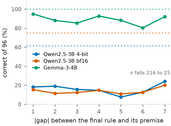
Figure 4: Accuracy against the gap between the final rule and the premise it fires on: all seven gaps, all three checkpoints, each checkpoint’s canonical-order score dashed. Distance is flat. Direction is not: rule-after scores 26.8, 22.4 and 94.9% against 5.8, 4.8 and 84.9% for rule-before. Gemma-3-4B still answers 84.9% of rule-before items correctly, so reversal degrades rather than prevents.
