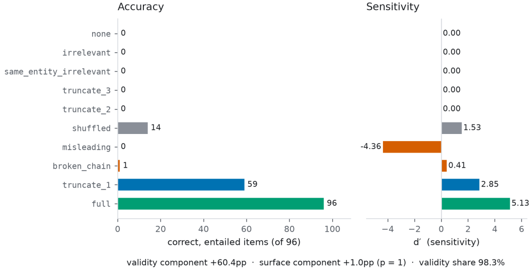
Figure 3: Ten matched arms on one item set, differing only in the solver record. Left: correct on the entailed subset (of 96). Right: sensitivity d' , signed. Destroying validity alone removes almost the whole effect on this checkpoint ; on gemma-3-4b it does not. The MISLEADING arm, whose fabricated final rule points the wrong way, is followed to the wrong answer on 189 of 192 items.
