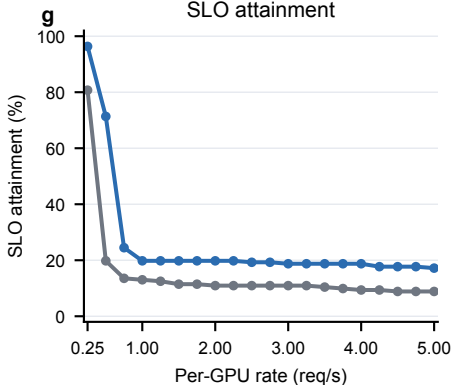
LLaMA2-13B + LongBench 4K SLO attainment
