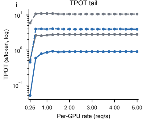
LLaMA2-13B + LongBench 4K TPOT tail
