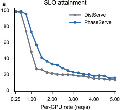
LLaMA2-13B + ShareGPT SLO attainment
