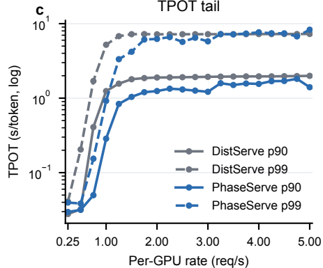
LLaMA2-13B + ShareGPT TPOT tail
