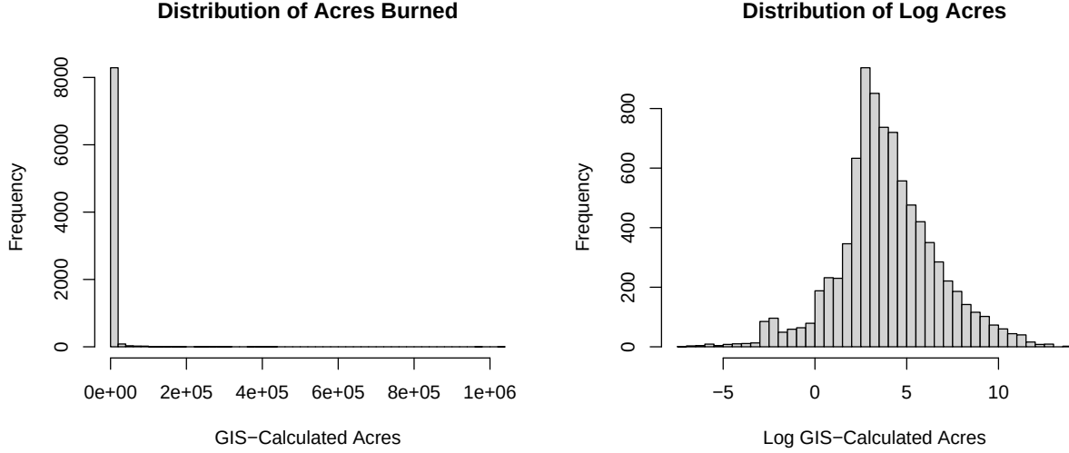
Figure 1: Raw and log-transformed acreage distributions.
