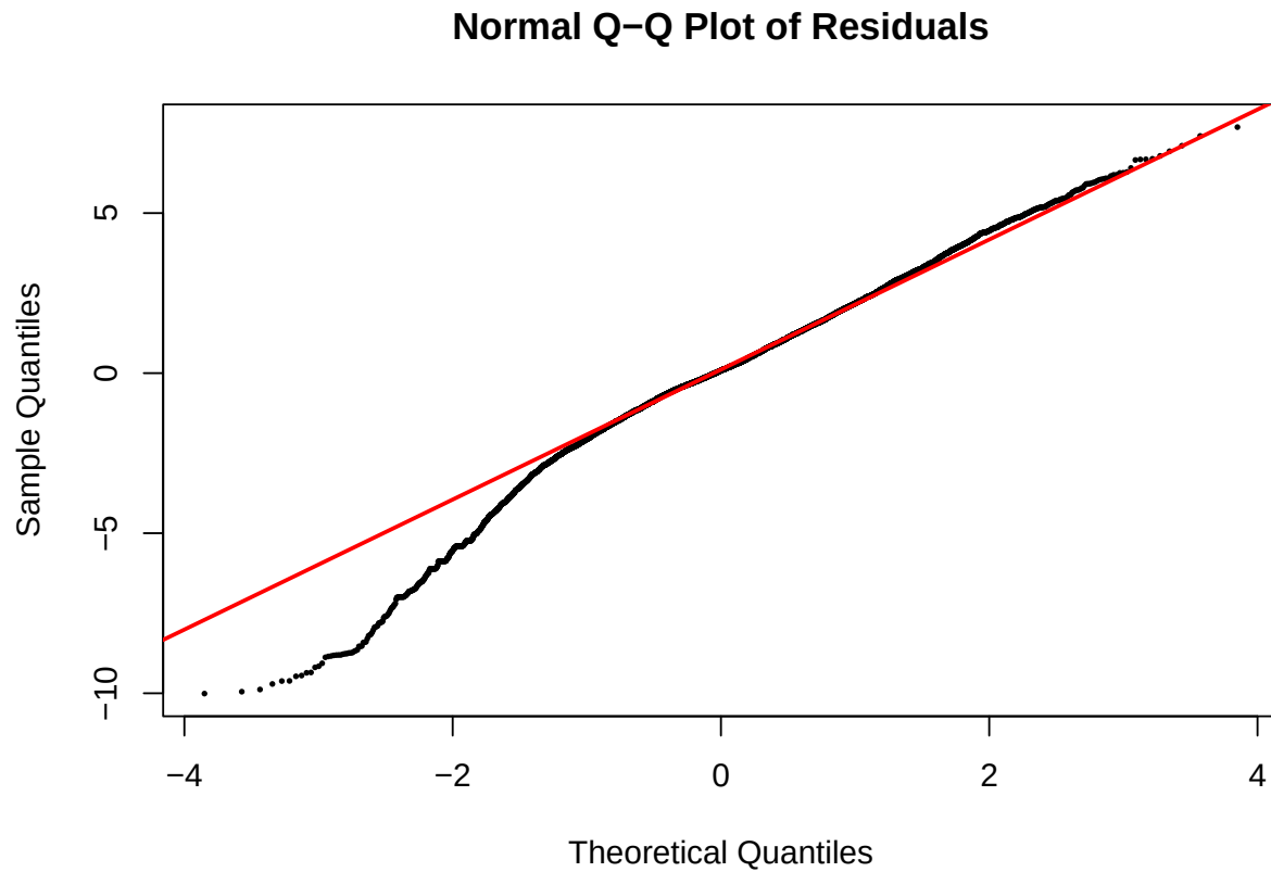
Figure 4: Normal Q-Q plot of the regression residuals.
