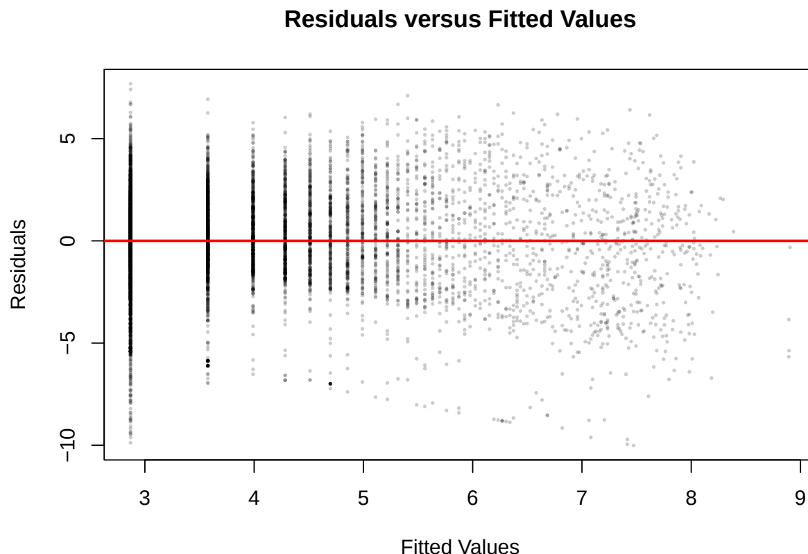
Figure 3: Residuals plotted against fitted values for the regression model.
