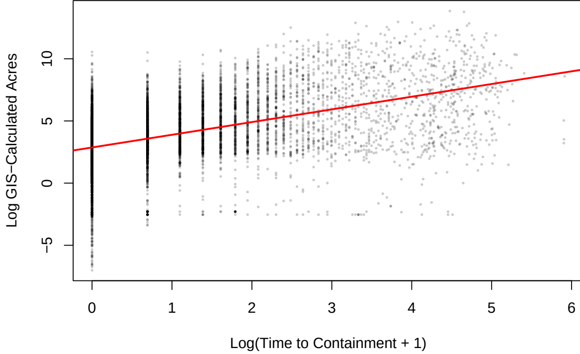
Figure 2: Log-transformed time to containment and log-transformed acreage, with the fitted regression line.
