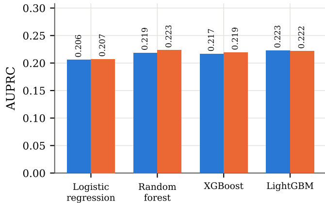
(b) Ranking of the positive class
