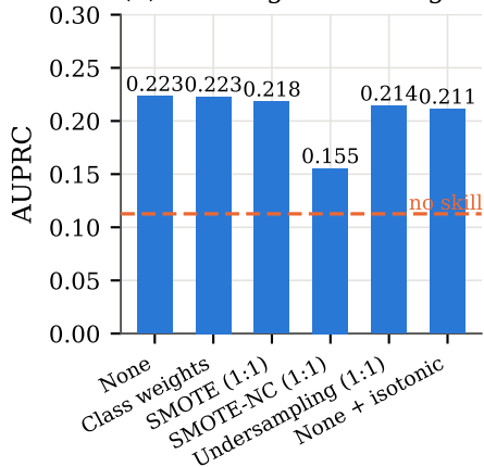
(a) Ranking is unchanged
