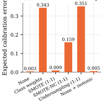
(b) Calibration is destroyed
