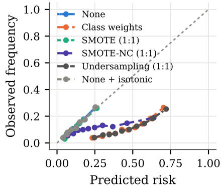
(c) Calibration curves
