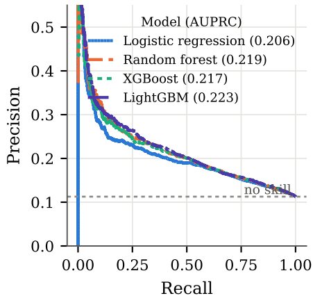
(b) Precision-recall
