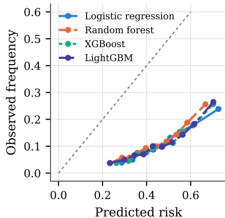
(c) Calibration
