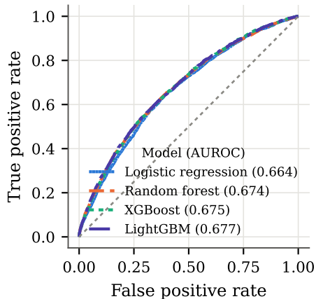
(a) ROC
