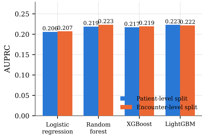
(b) Ranking of the positive class
