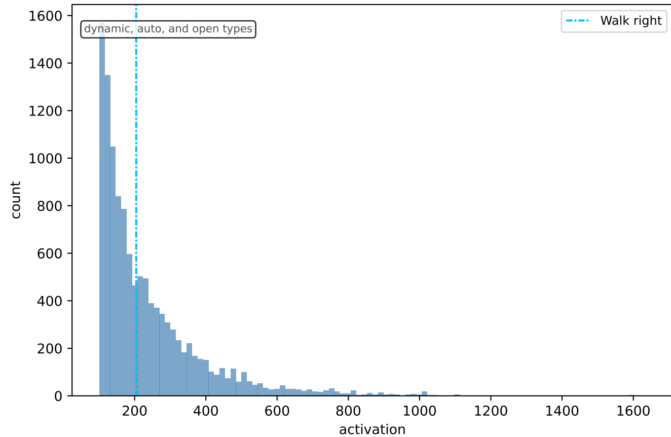
SAE 603 — Context (non-zero)
