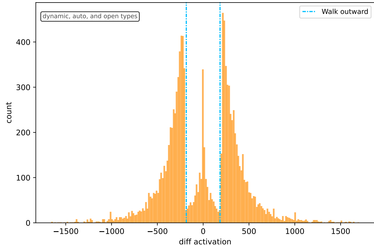
SAE 603 — Diff (non-zero)
