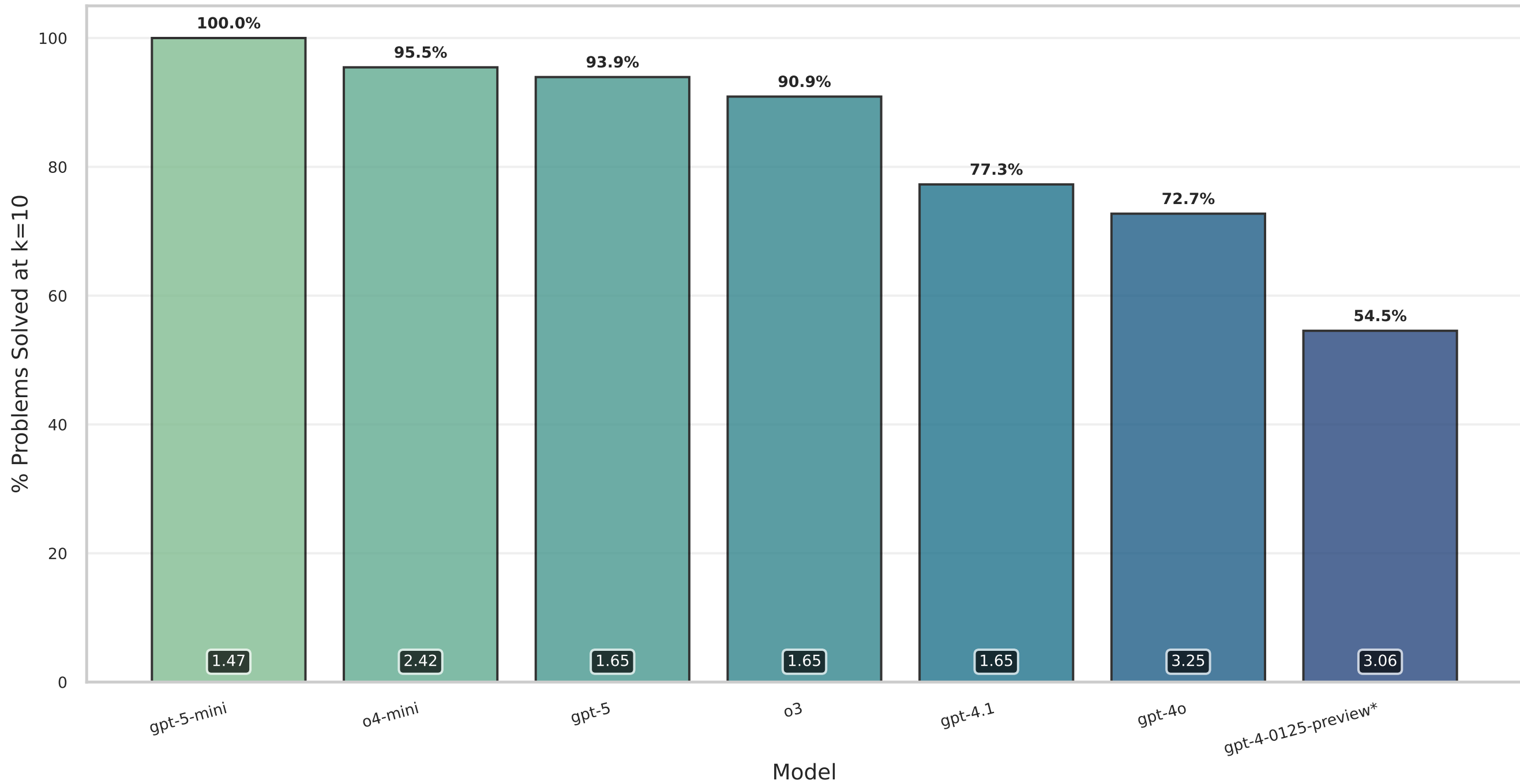
Model Performance: % Solved at k=10 with Average Attempts (Averaged across runs)
