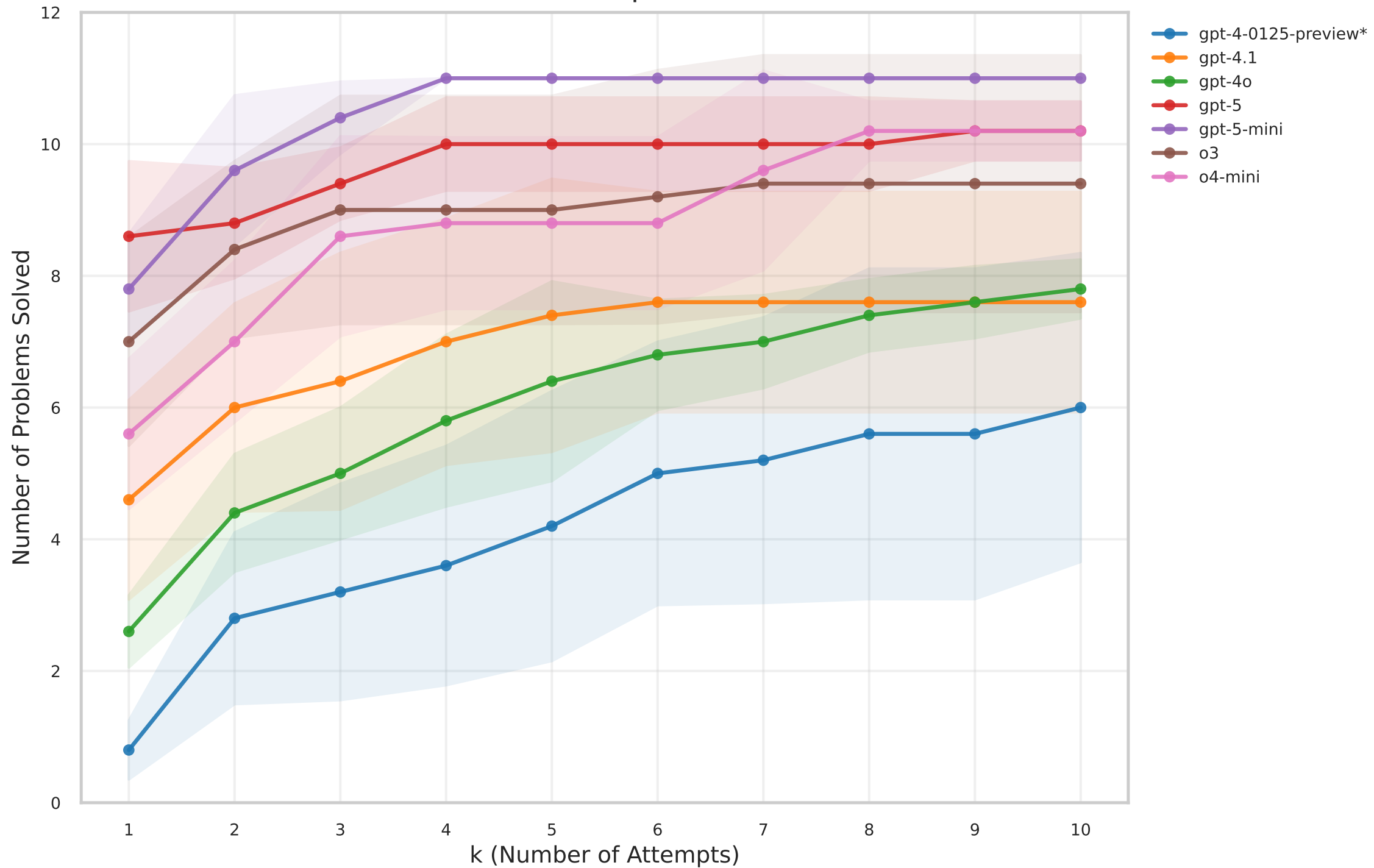
Solved at k - Model Comparison (Mean \pm SD)
