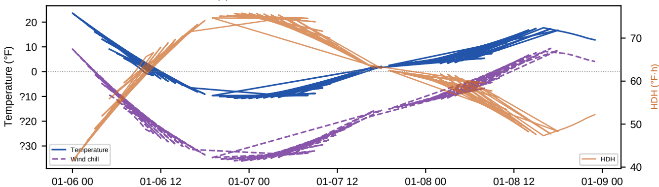
(c) ERA5 Great Lakes core weather, Jan 6–8
