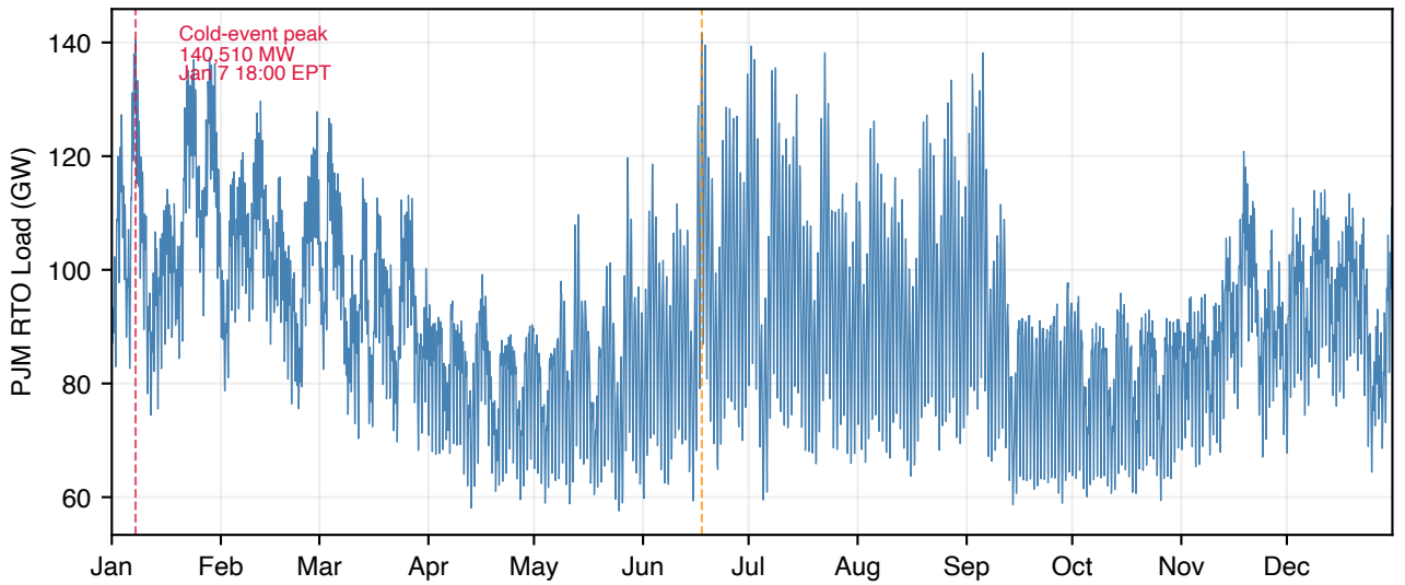
(a) Full-Year 2014 PJM RTO Hourly Load
