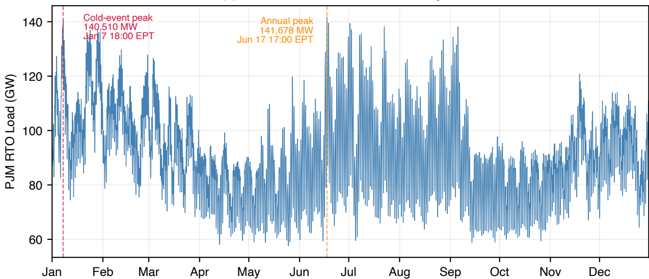
(a) Full-Year 2014 PJM RTO Hourly Load
