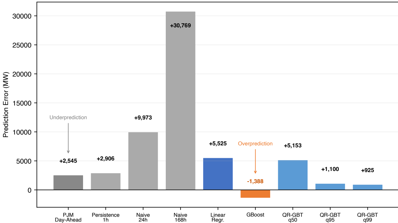
Event Peak Prediction Errors, Jan 7 18:00 EPT (Actual = 140,510 MW)
