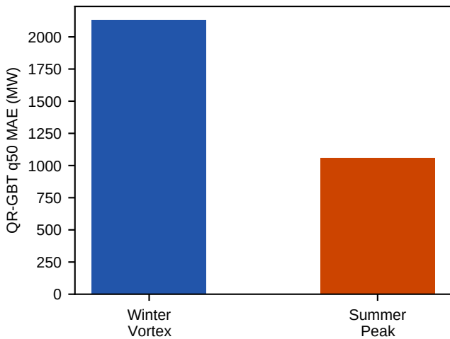
(c) Point forecast error
