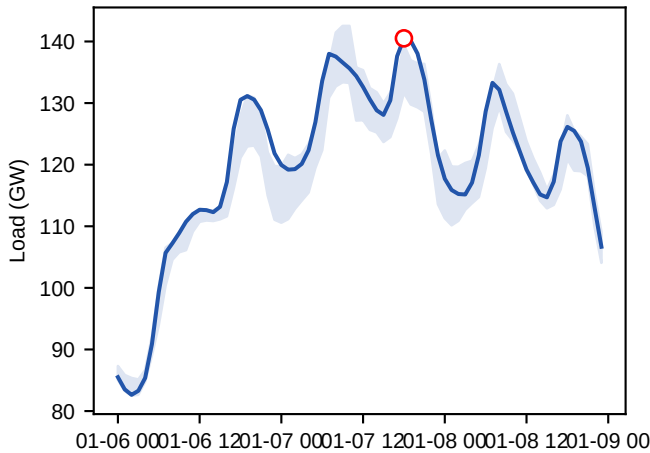
(c) Point forecast error
