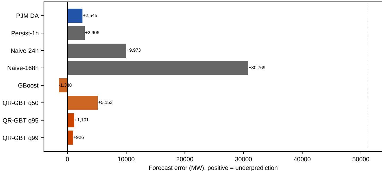
Prediction errors at Jan 7 18:00 event peak (140.5 GW)
