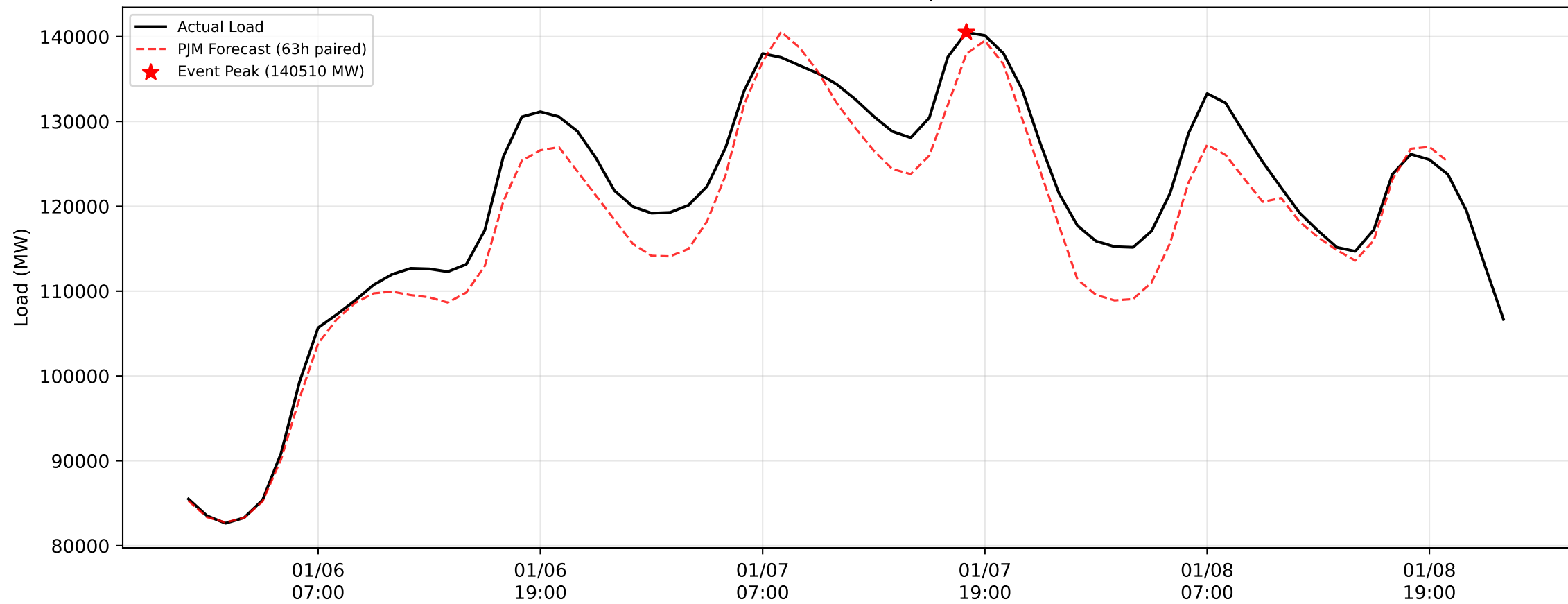
2014 Polar Vortex — 63/72 paired hours
