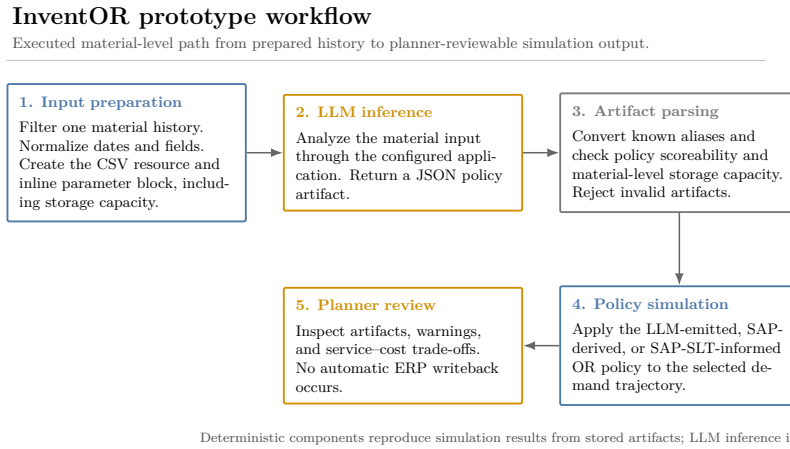
Figure 1: InventOR workflow: material data are prepared, an LLM proposes a policy, deterministic software parses, checks and simulates it, and a planner reviews the result.
