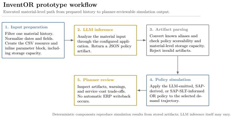
Figure 1: InventOR workflow: material data are prepared, an LLM proposes a policy, deterministic software parses, checks and simulates it, and a planner reviews the result.
