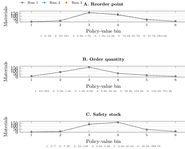
Figure 4: Distribution of the proposed reorder point (A), order quantity (B) and safety stock (C) over the 365 materials in the three runs, on common log-spaced bins. Nearly coinciding lines show reproducible aggregate behaviour.
