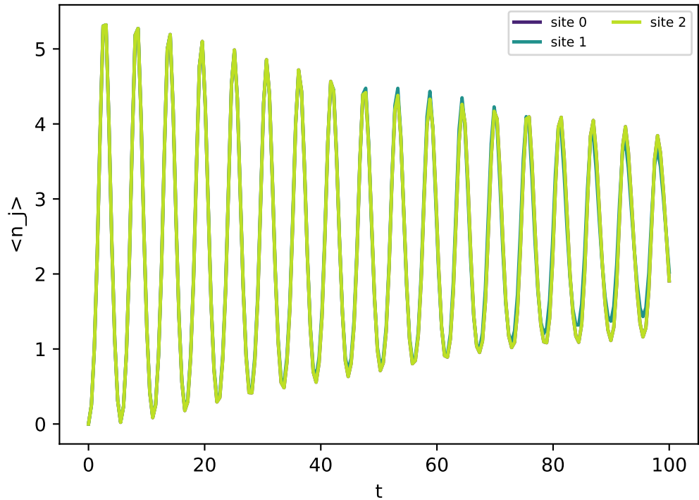
Boson occupation
