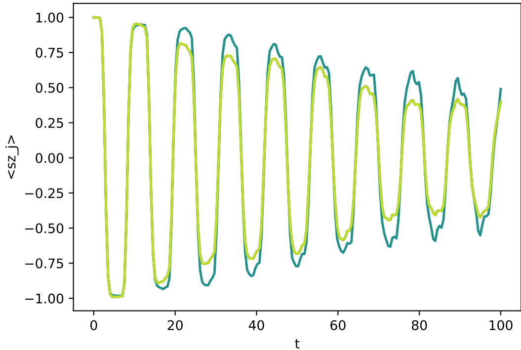
Spin magnetization
