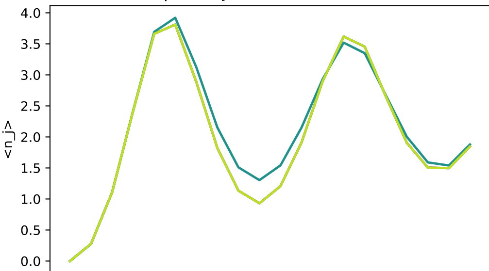
Boson occupation, J=2 , truncation error= 5.82\text{e-}05
