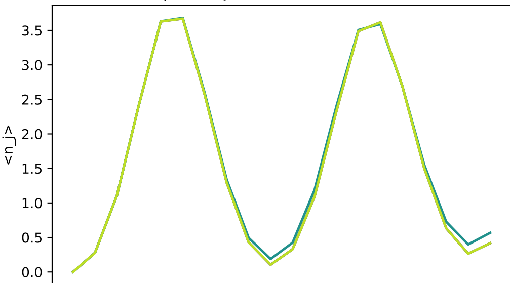
Boson occupation, J=0.5 , truncation error= 5.20\text{e-}05
