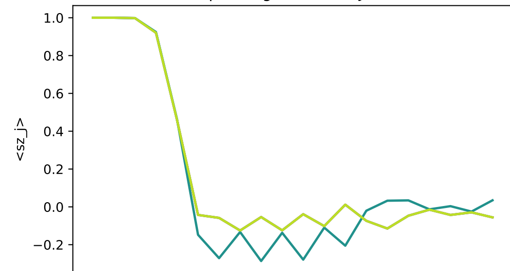
Spin magnetization, J=2
