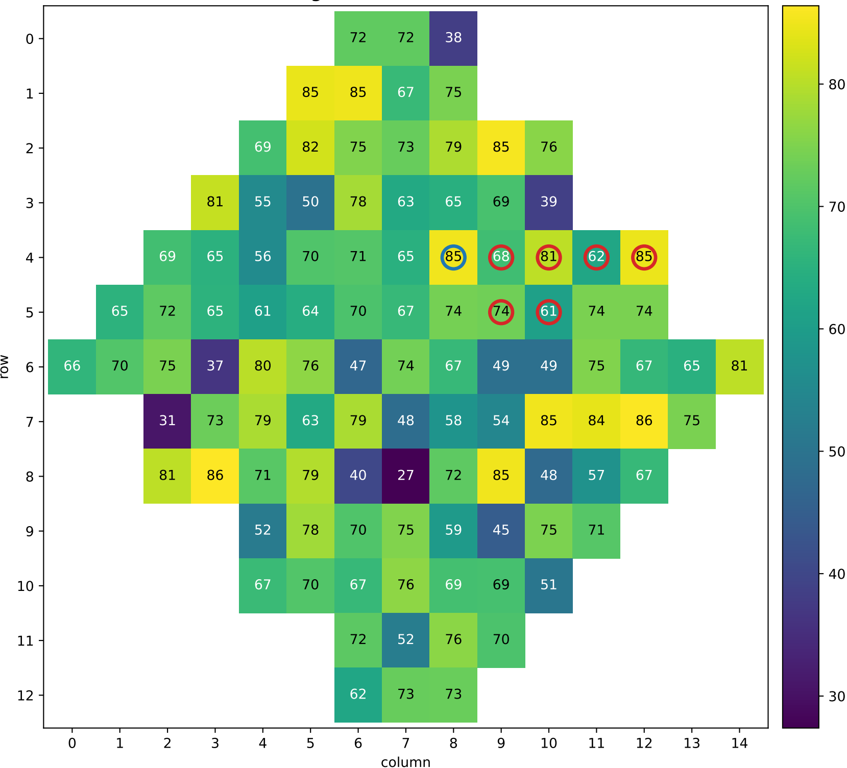
Single Qubit Idle T1 Micros
