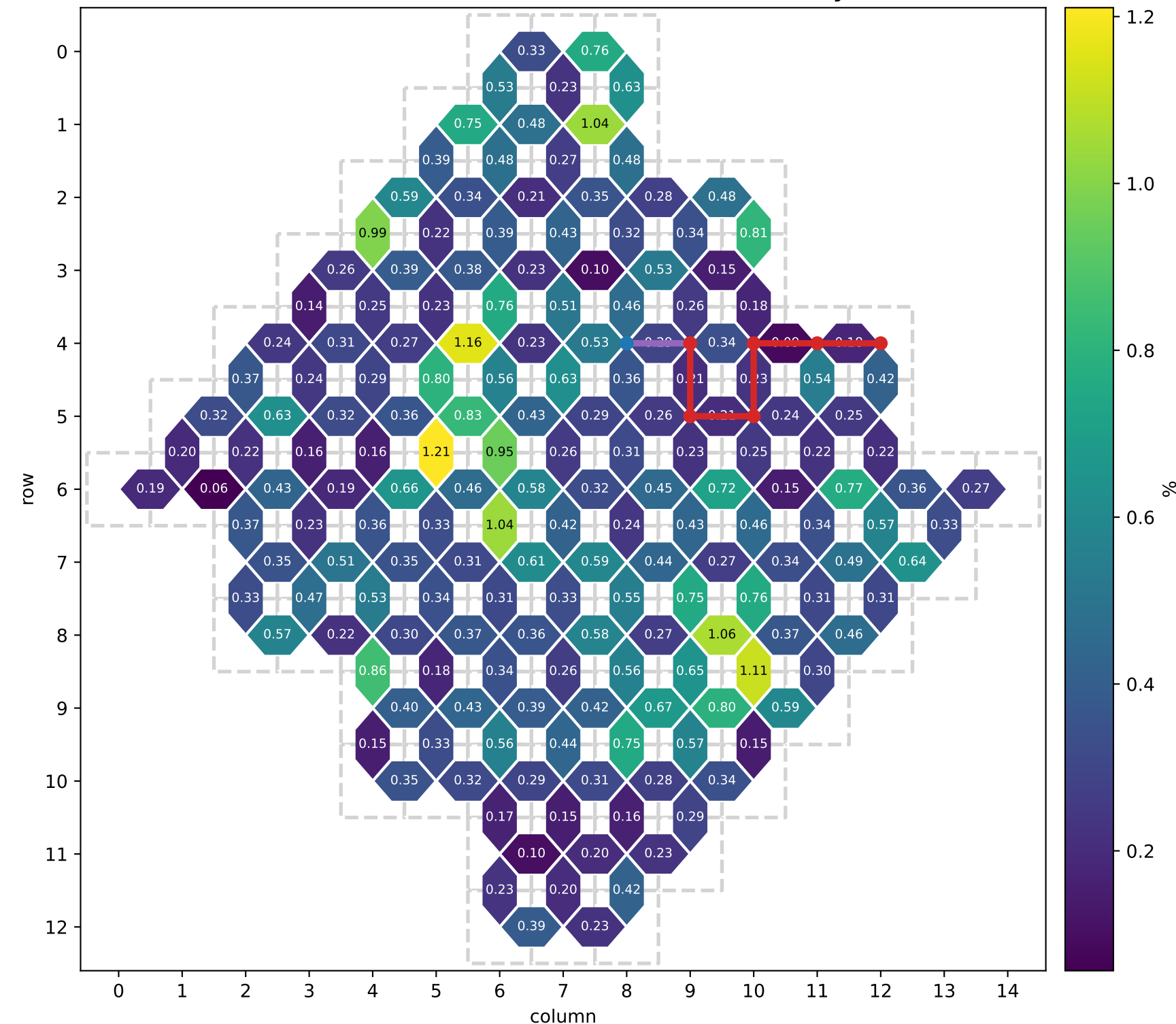
Two Qubit Parallel Cz Gate Xeb Pauli Error Per Cycle
