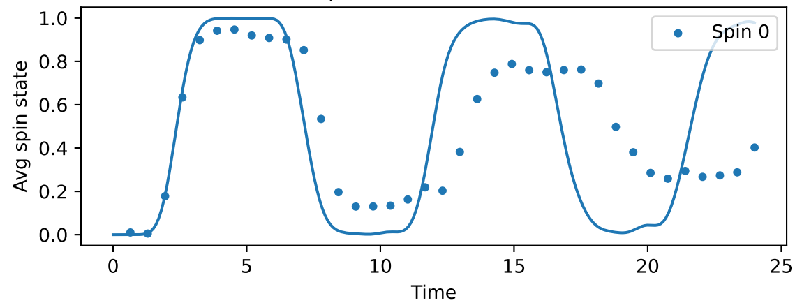
Timesteps=37, Trotter time=0.649
