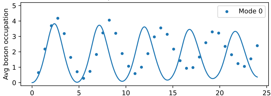
Timesteps=36, Trotter time=0.667
