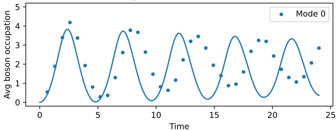
Timesteps=37, Trotter time=0.649
