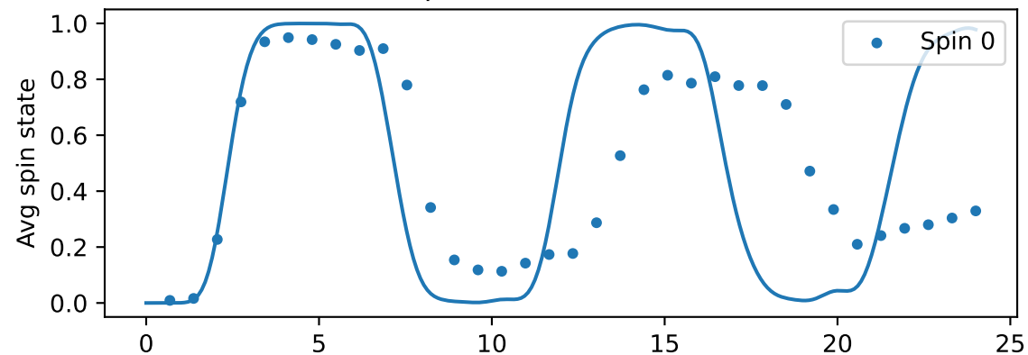
Timesteps=36, Trotter time=0.667
