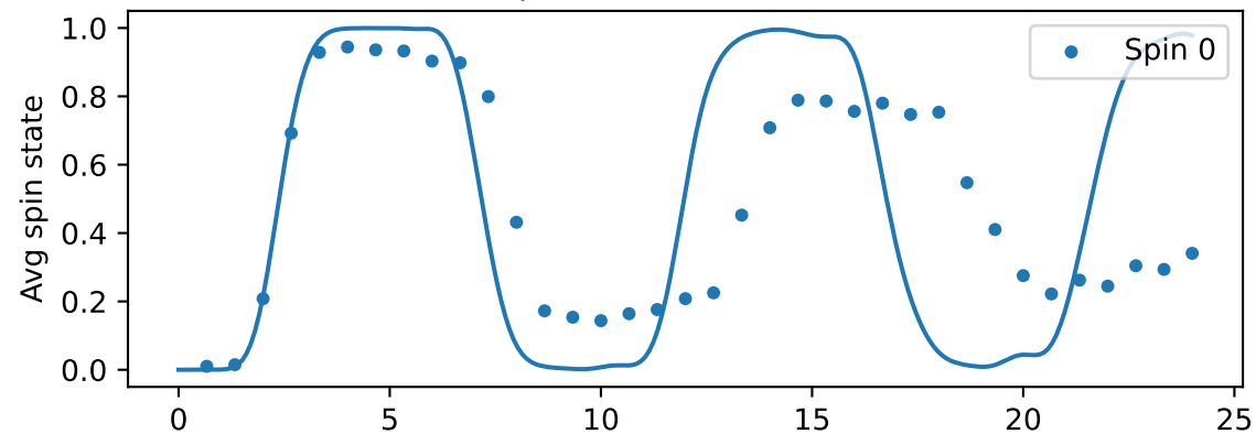
Timesteps=37, Trotter time=0.649
