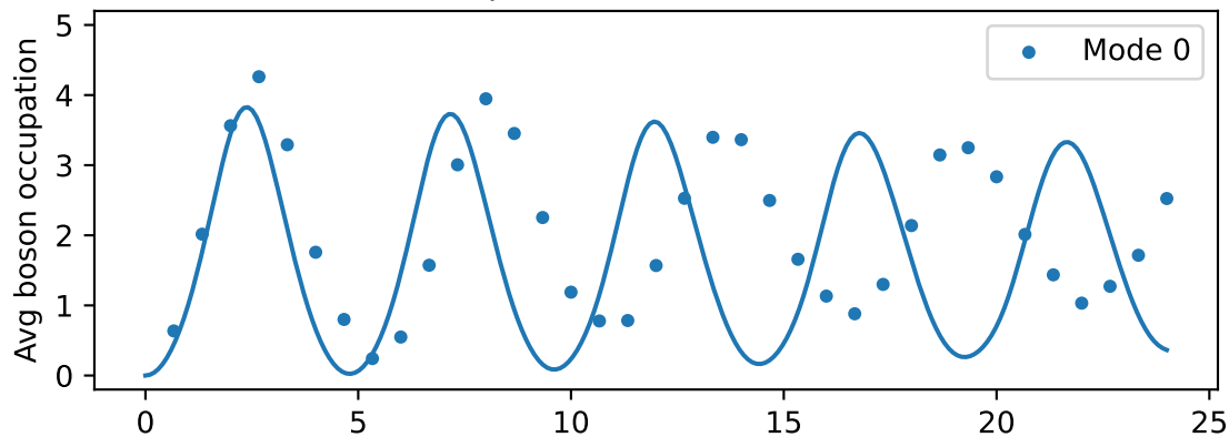
Timesteps=37, Trotter time=0.649
