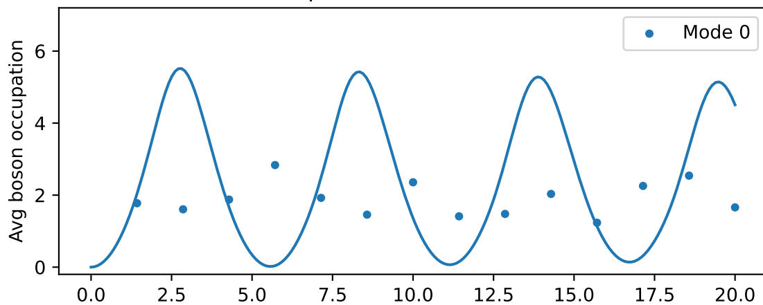
Timesteps=14, Trotter time=1.429
