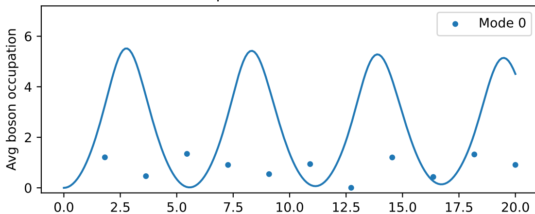
Timesteps=12, Trotter time=1.667
