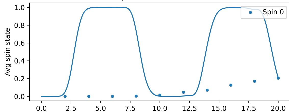
Timesteps=11, Trotter time=1.818
