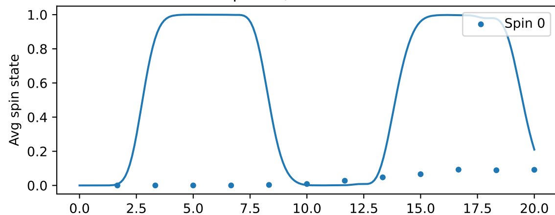
Timesteps=13, Trotter time=1.538
