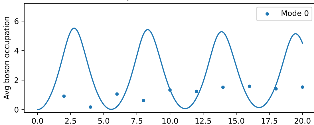
Timesteps=11, Trotter time=1.818
