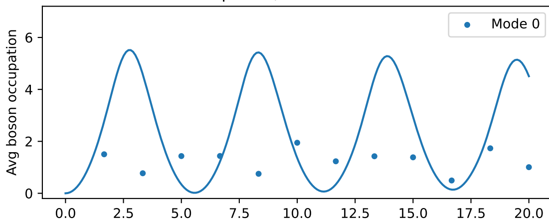
Timesteps=13, Trotter time=1.538
