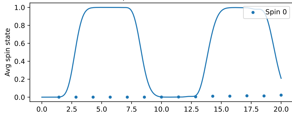
Timesteps=14, Trotter time=1.429
