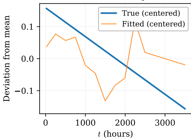
(a) Trend (corr = 0.200, slope ratio = 0.13)
