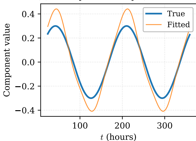
(c) Weekly seasonality (corr = 0.996)
