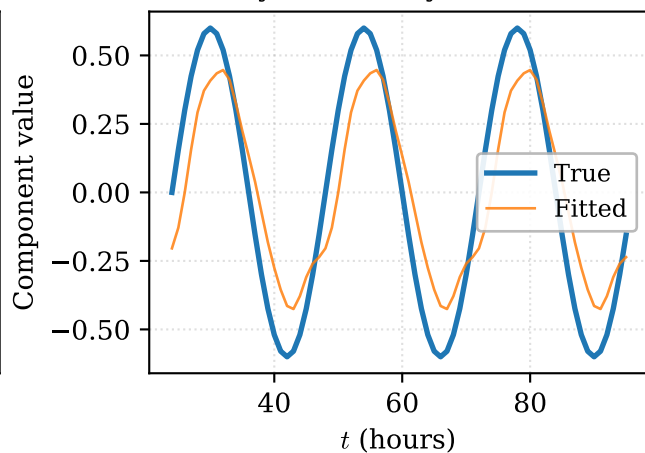
(b) Daily seasonality (corr = 0.926)
