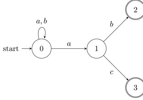
Figure 15: NFA \mathcal{A} over \Sigma = \{a, b, c\}
